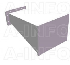
LB-510-10-ASPO Standard Gain Horn Antenna 1.45-2.2GHz 10dB Gain Rectangular Waveguide Interface
