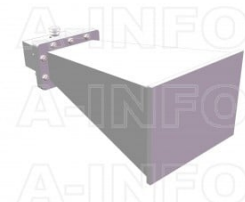
LB-510-10-C-7/16FSPO Standard Gain Horn Antenna 1.45-2.2GHz 10dB Gain 7/16(DIN) Female
